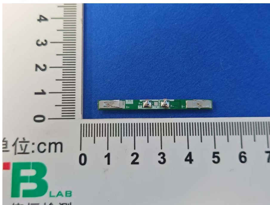
Picture 6. Back view of protection board
