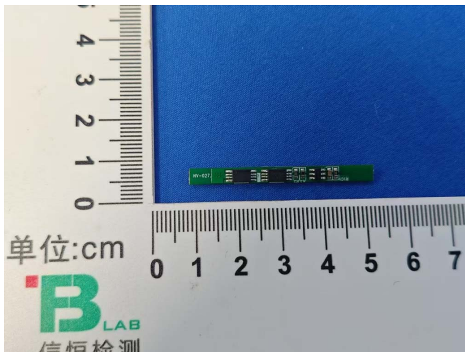
Picture 5. Front view of protection board
